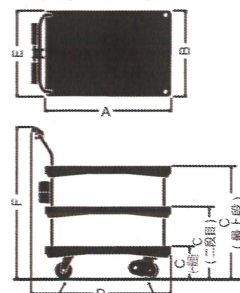
■寸法図(ASP-300-T3)
