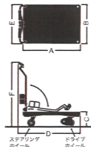
■寸法図(ASP-300-T3)
